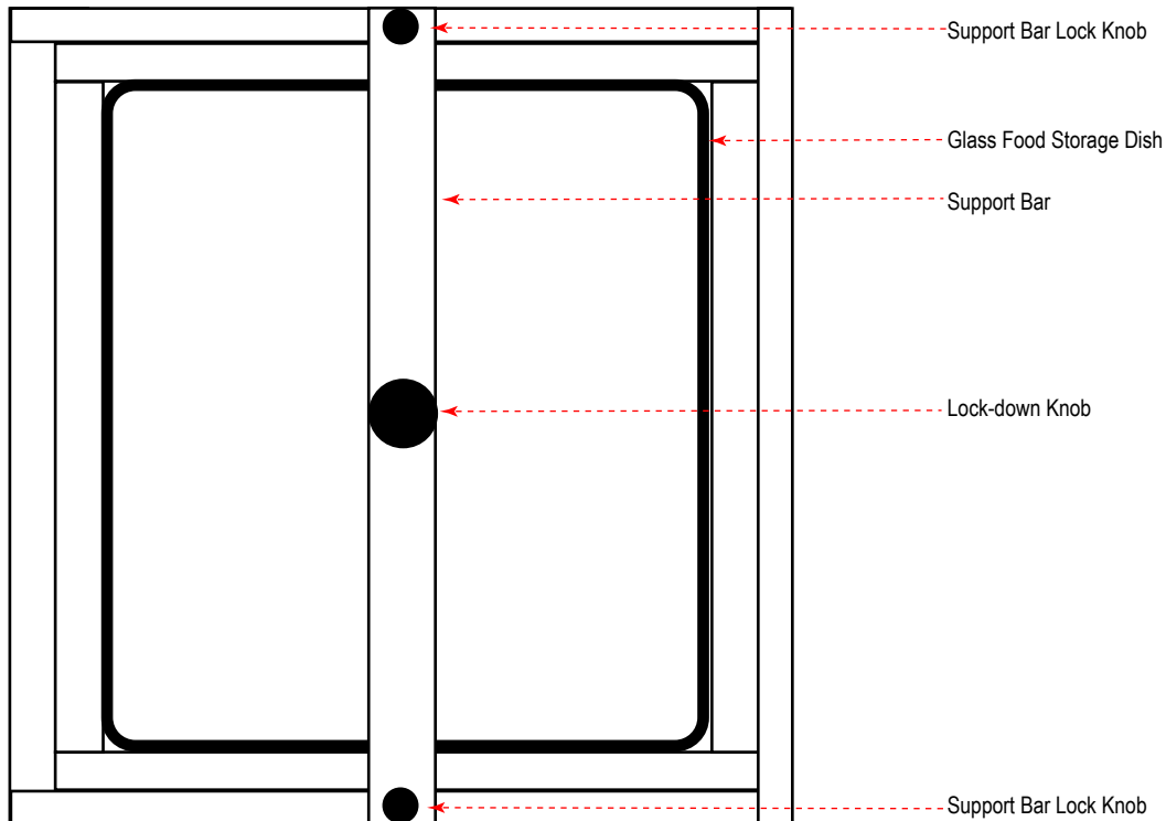
Fuming Box top view
